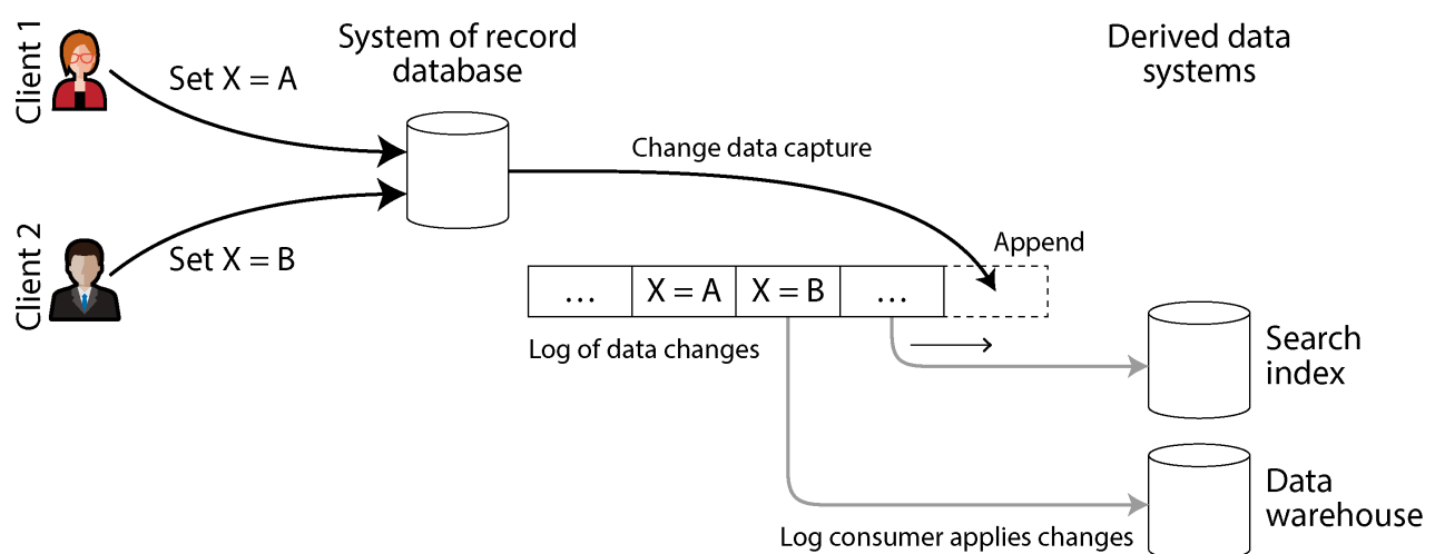
Figure 12-5. Taking changes committed to a database and propagating them to downstream systems in the same order
