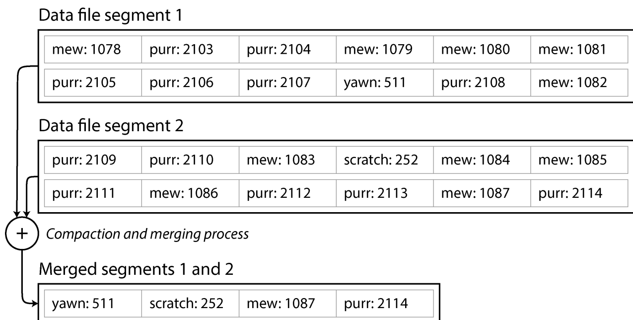
Figure 12-6. In this log of key-value pairs, the key is the ID of a cat video (mew, purr, scratch, or yawn) and the value is the number of times it has been played; log compaction retains only the most recent value for each key.
